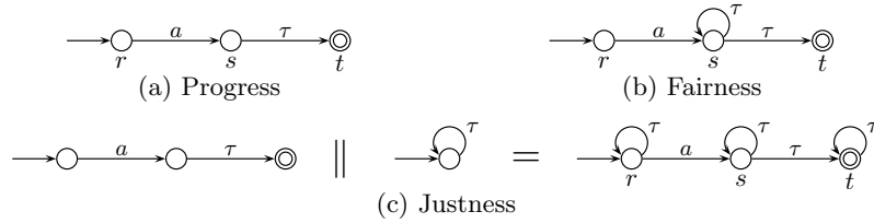
Fig. 1. Progress, Fairness and Justness
